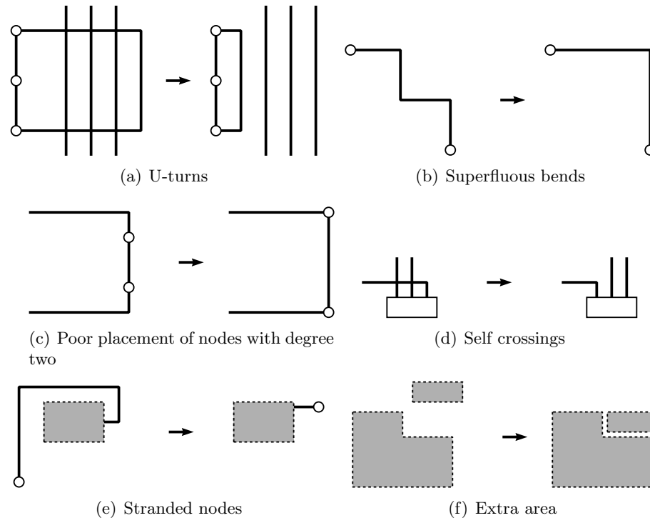
Figure 2.22: Examples of particular problems when drawing orthogonal embeddings of graphs. These problems are dealt with by refinement [SKT00].
