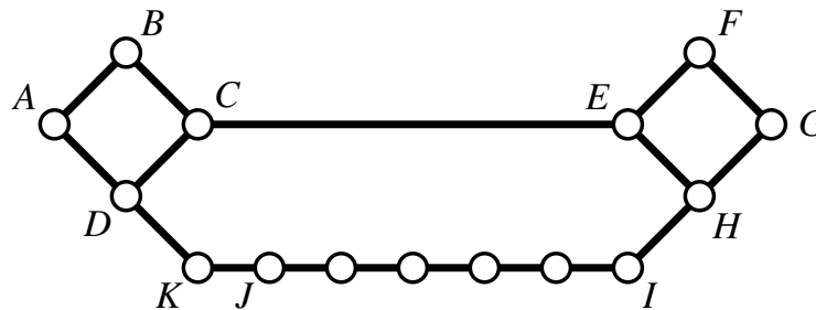
Figure 4.5: Example of failed clustering with overlenth edges.
