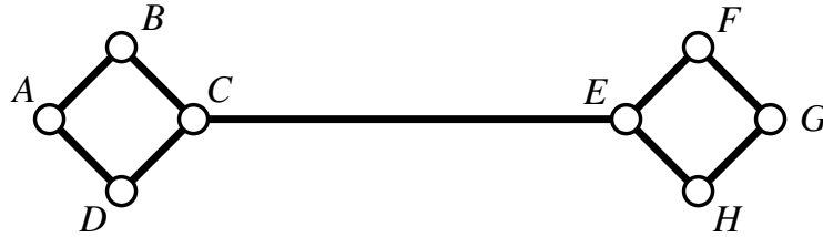
Figure 4.2: Example of clustering with a single overlenth edge. An attempt to cut the graph based on the edge CE will produce two clusters of nodes: \{A, B, C, D\} and \{E, F, G, H\}
