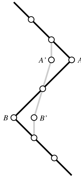
Figure 5.12: A second example of a local minimum involving a conflict between the octilinearity and line straightness criteria.
