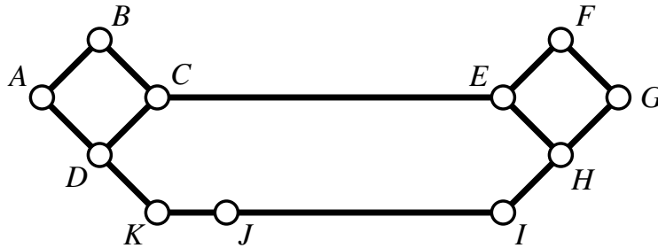
Figure 4.3: Example of failed clustering with a single overlenth edge. In this case, cutting the graph based on the edge CE will not find two clusters of nodes.
