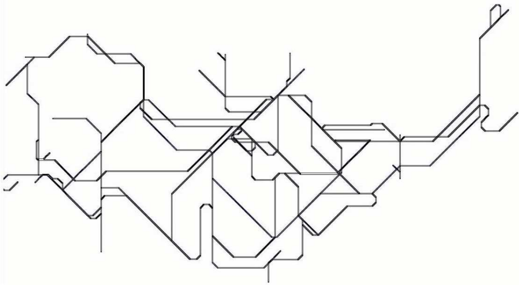
Figure 2.46: The London Underground map as drawn by Merrick and Gudmundsson [MG07].
