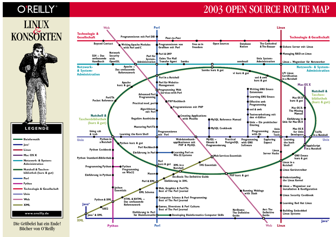
Figure 2.37: Open source route map [ORe].
