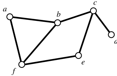
Figure 2.14: [An embedding of] a graph. The graph, G , contains a set of nodes, V = \{a, b, c, d, e, f\} , and a set of edges, E = \{\{a, b\}, \{b, c\}, \{c, d\}, \{c, e\}, \{e, f\}, \{b, f\}, \{a, f\}\} .
