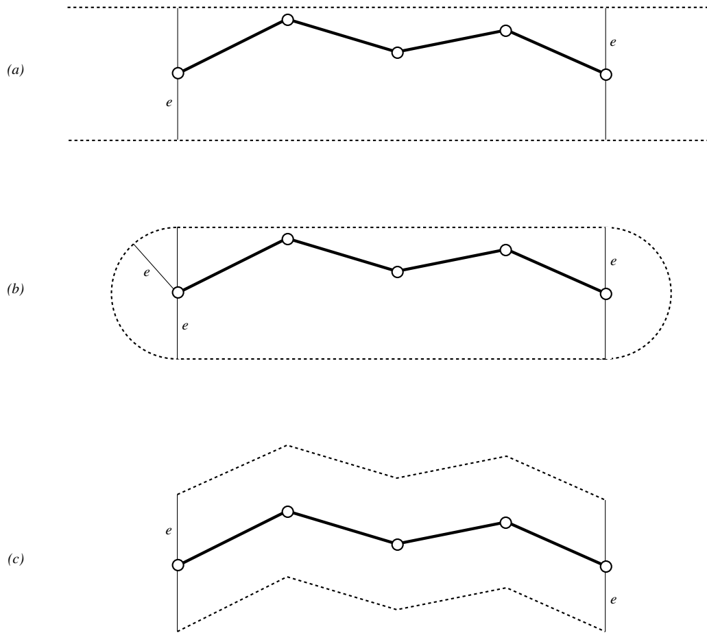
Figure 2.25: Illustration of different line generalisation error criteria. Bounds of errors are shown with dashed lines; e is the acceptable magnitude of the error. Line (a) shows the parallel-strip (or infinite beam) criterion; line (b) shows the tolerance zone criterion; line (c) shows the uniform metric criterion.
