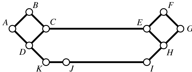
Figure 4.3: Example of failed clustering with a single overlenght edge. In this case, cutting the graph based on the edge CE will not find two clusters of nodes.
