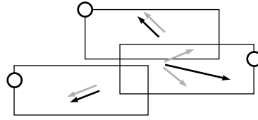
Figure 2.33: Example of overlap vectors for labelling using Hirsch's algorithm. The grey arrows indicate the individual overlap vectors from each label overlap; the black arrows indicate the aggregate overlap vectors for each label.
