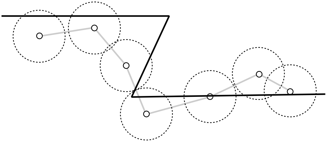
Figure 2.43: Path simplification by stabbing \epsilon -circles. The line being simplified is shown in grey with \epsilon -circles shown with dotted lines. A simplified line that stabs all the \epsilon -circles is also shown.
