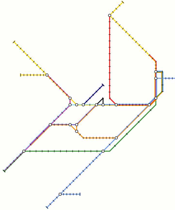
Figure 2.36: The Sydney CityRail map as drawn by Nöllenburg [N05].
