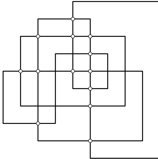
Figure 2.19: An embedding of an orthogonal embedding of a graph.
