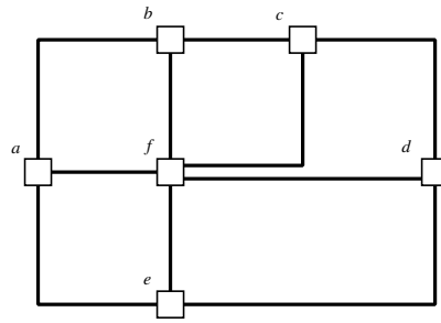
Figure 2.21: An embedding of a nearly orthogonal embedding of a graph [FK95].
