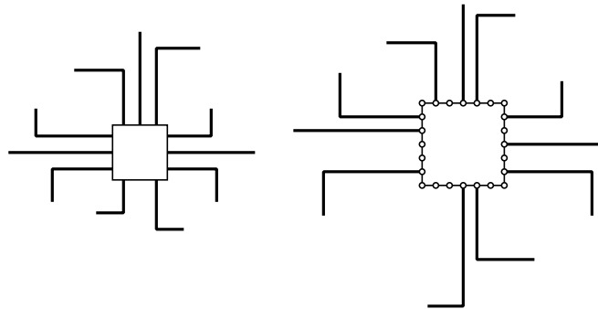
Figure 2.22: An example of replacing a large node with high degree with 8s smaller nodes.
