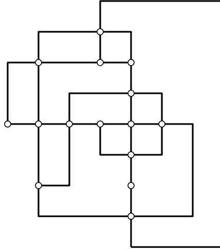
Figure 2.20: An embedding of a planar orthogonal embedding of a graph.
